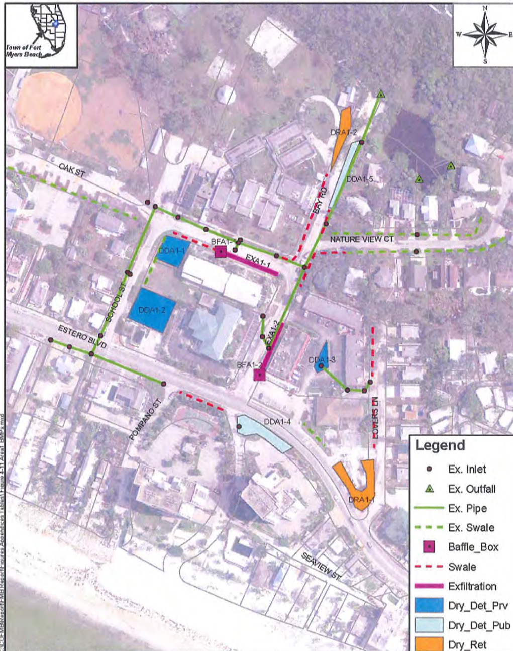
Figure ES-5 Proposed BMPs Area 1 Estero Boulevard & Bay Road
